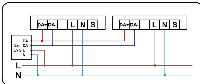
Master-Master-Anschluss Master-Master connection
